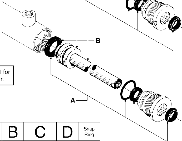
SINGLE-ACTING CYLINDER
